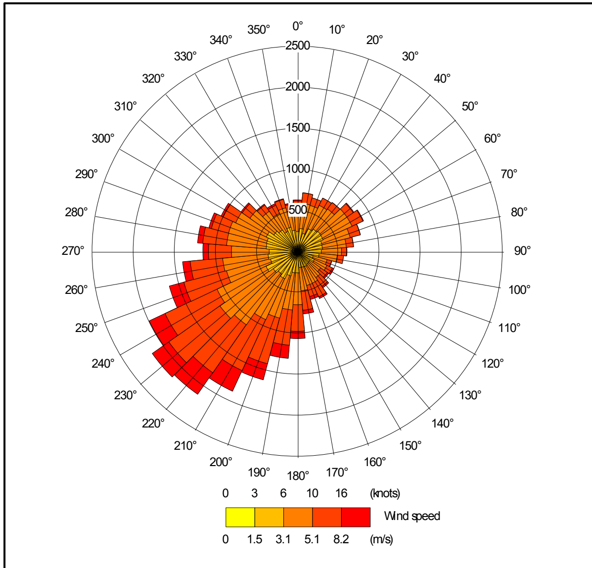
Figure 3a. The wind rose. Raw GFS derived data for 52.916 N, 1.001 W, 2013 – 2016
