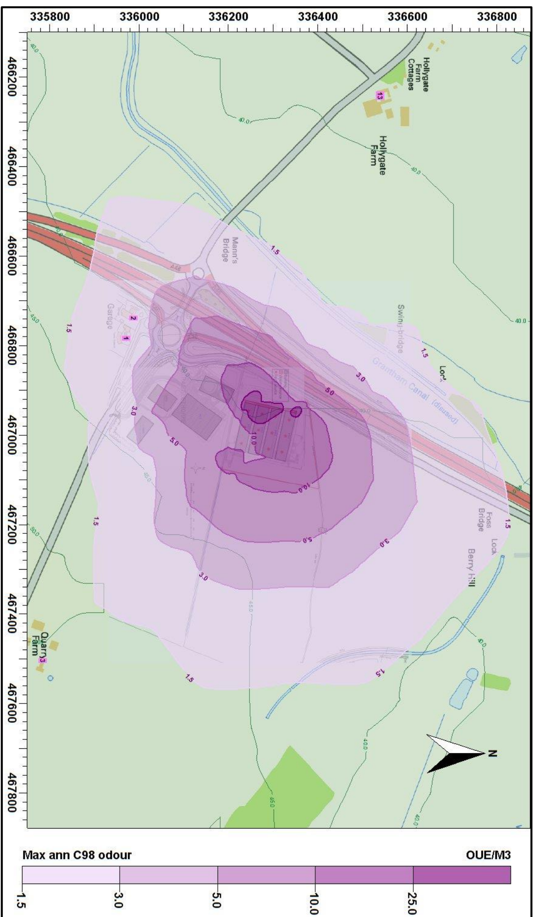
Figure 6. Predicted maximum annual 98 th percentile hourly mean odour concentration
