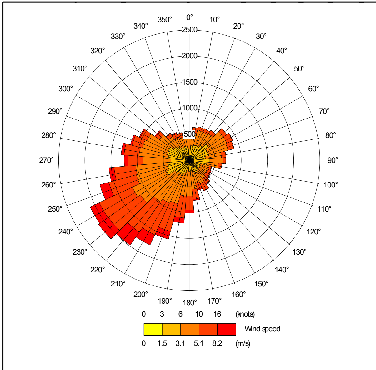
Figure 3b. The wind rose. FLOWSTAR modified GFS derived data for NGR 467000, 336300
